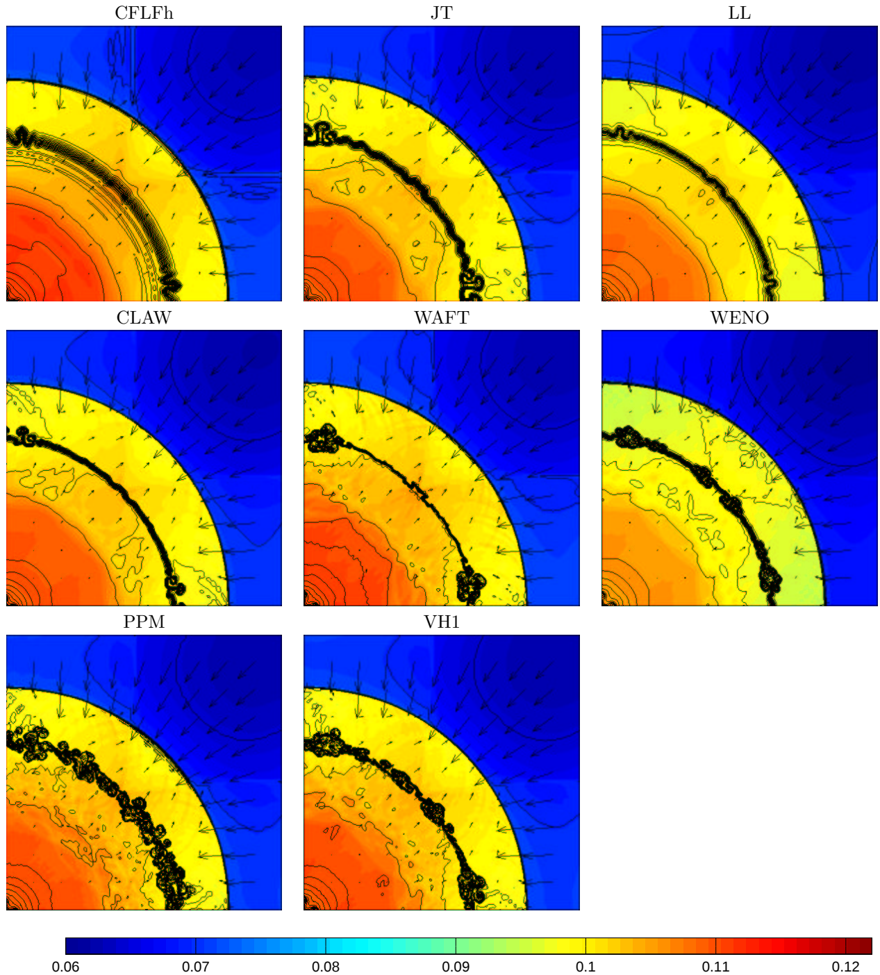
FIG. 4.12. Results for the explosion problem by all eight schemes. Color pressure map is overlayed by 27 density contours (0.08 to 0.21 step 0.005) and velocity arrows. Computations were done on the square (x, y) \in (0, 1.5) \times (0, 1.5) with 400 \times 400 grid till time T = 3.2 .
