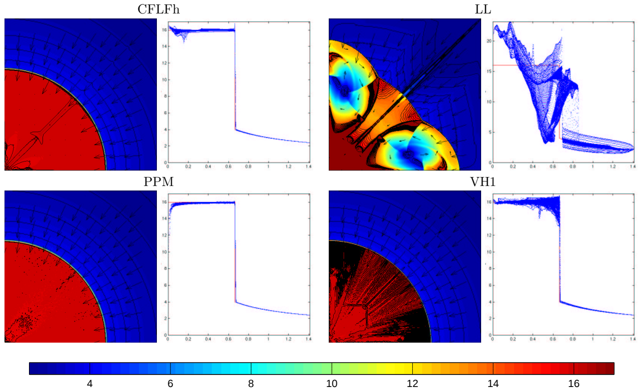
FIG. 4.7. Results for the Noh problem by the CFLFh, LL, PPM and VH1 schemes. JT, CLAW, WAF and WENO have failed for this problem. Density color map is overlaid by 23 density contours ( 2.5 to 4 step 0.25 and 14 to 17 step 0.2) and velocity arrows on the left. Scatter plot of density versus radius is on the right. The computations were done on the square (x, y) \in (0, 1) \times (0, 1) with 400 \times 400 grid to time T = 2 .
