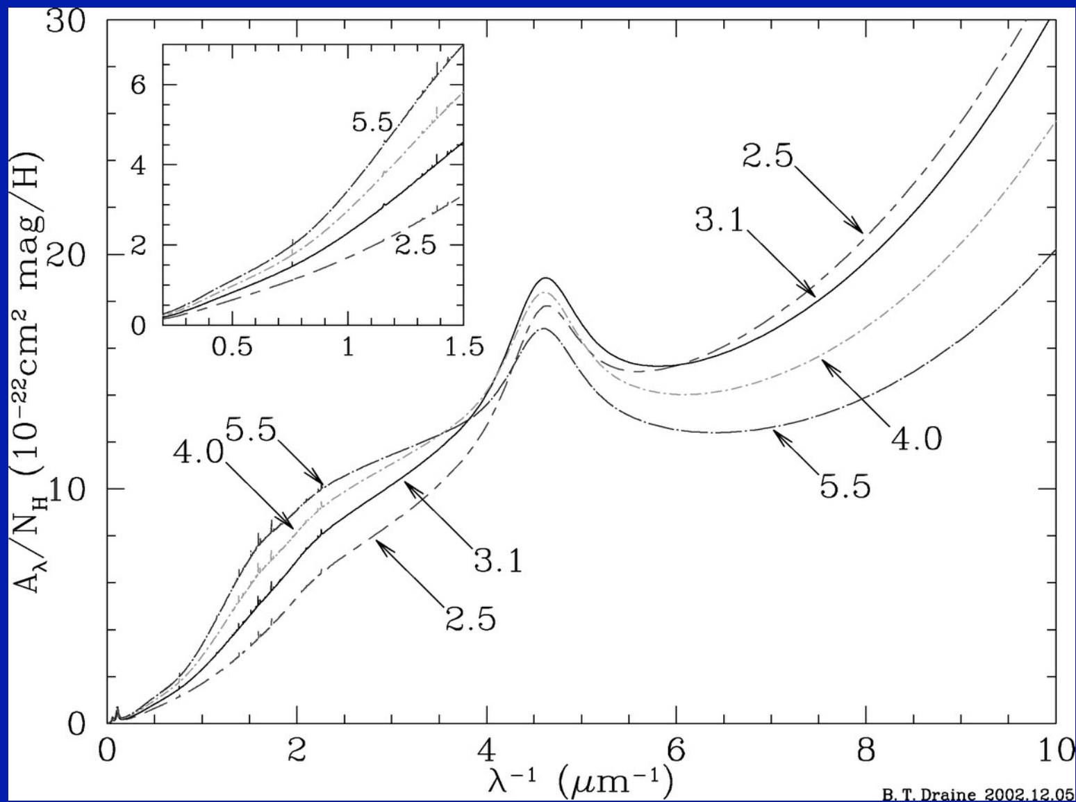
Extinction curves from Draine (2003)
