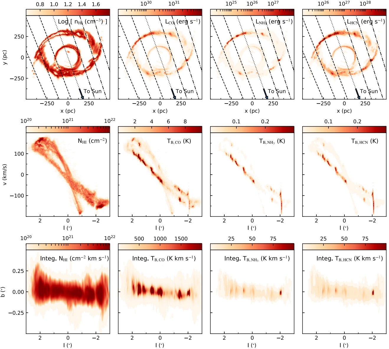
Figure 5. Top panels: from left to right snapshots taken at z = 0 of H I number density, n_{\text{HI}} , CO ( J = 1 - 0 ) luminosity, L_{\text{CO}} , NH 3 (1,1) luminosity, L_{\text{NH}_3} , and HCN ( J = 1 - 0 ) luminosity, L_{\text{HCN}} . The bar major axis is aligned with the axis x = 0 . In each plot, the dotted black line indicates the line connecting the Sun to the Galactic Centre, l = 0 , while the dashed/dot-dashed line indicate the line of sights at l = \pm 1^\circ, 2^\circ, 3^\circ . The arrow points towards the Sun position. Central panels: from left to right longitude–velocity distributions of H I column density, N_{\text{HI}} , CO ( J = 1 - 0 ) brightness temperature, T_{\text{CO}} , NH 3 (1,1) brightness temperature, T_{\text{NH}_3} , and HCN ( J = 1 - 0 ) brightness temperature, T_{\text{HCN}} , averaged over the latitude range \pm 0.5^\circ . Bottom panels: from left to right ( l, b ) maps of N_{\text{HI}} , T_{\text{CO}} , T_{\text{NH}_3} , and T_{\text{HCN}} , integrated over the velocity range \pm 200 \text{ km s}^{-1} . The gas distribution is analysed at t = 505 \text{ Myr} .
