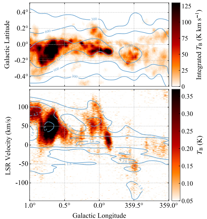
Figure 1. Distribution of \text{NH}_3 (1,1) (heat colour-scale, Walsh et al. 2011; Purcell et al. 2012) and \text{CO} ( J = 1 - 0 ) (blue contours, Bitran et al. 1997; Dame et al. 2001) emission in the central 2^\circ of the Galaxy. The upper panel shows the integrated brightness temperature map over a velocity range \pm 350 \text{ km s}^{-1} , while the lower panel shows the longitude–velocity diagrams averaged over latitude \pm 0.5^\circ .
