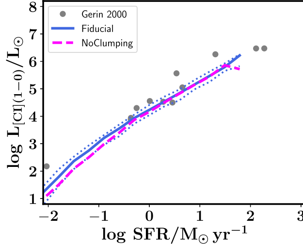
Figure B4. The [C I] 1–0 luminosity of galaxies at z = 0 as a function of their SFR for a model variant with (Fiducial) and without (NoClumping) turbulence-dependent clumping. This figure is similar to Fig. 9. Clumping has a minimal effect on the predicted [C I] luminosities of galaxies.
