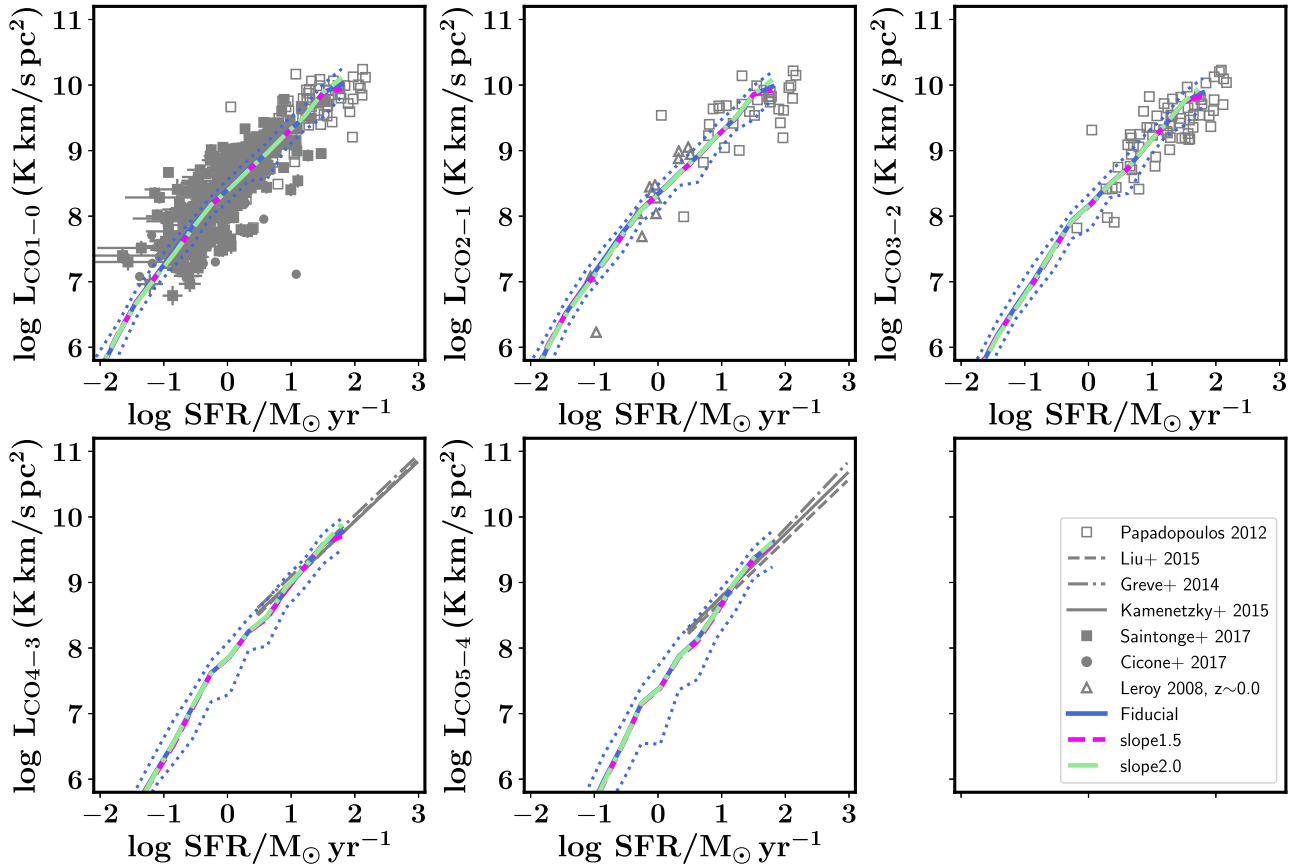
Figure C2. The CO J=1–0 to 5–4 luminosity of galaxies as a function of their SFR at z = 0 for a model variant with a slope \beta of the cloud mass distribution function of \beta = 1.8 (Fiducial), \beta = 1.5 (slope1.5), and \beta = 2.0 (slope2.0). This figure is similar to Fig. 7. Different choices for the slope of the molecular cloud mass distribution function do not affect the predicted CO luminosity of galaxies.
