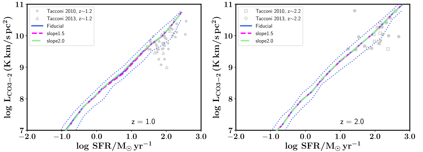
Figure C3. The CO J=3–2 luminosity of galaxies at z = 1 and 2 as a function of their SFR for a model variant with a slope \beta of the cloud mass distribution function of \beta = 1.8 (Fiducial), \beta = 1.5 (slope1.5), and \beta = 2.0 (slope2.0). This figure is similar to Fig. 8. Different choices for the slope of the molecular cloud mass distribution function do not affect the predicted CO luminosity of galaxies.
