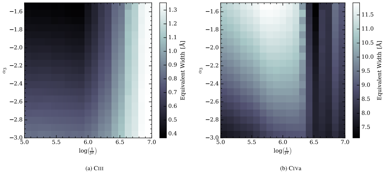
Figure 3. 2D plots of equivalent width versus changes in cluster age or IMF slope for two spectral regions (C III and C IV \lambda ), where the equivalent width reported for a grid cell is the median of the equivalent widths for the clusters that reside in that area of parameter space. In both panels, we see that the equivalent width of these lines may be used to differentiate the various possible values of \alpha_3 at young ages. In addition, the combination of the two lines provides us with a way to also differentiate the age of the cluster in conjunction with the value of \alpha_3 .
