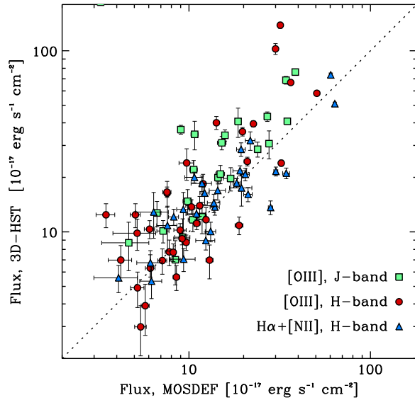
Figure 10. Comparison of emission-line fluxes as measured from MOSDEF and 3D-HST. We consider lines with an S/N > 3 in both the MOSDEF and 3D-HST spectra. Because of the lower spectral resolution of the 3D-HST grism spectra, we combine H \alpha and the two [N II] lines and the two [O III] lines for MOSDEF. The flux measurements for both surveys are corrected to the total flux by scaling the spectra to the 3D-HST photometry.
