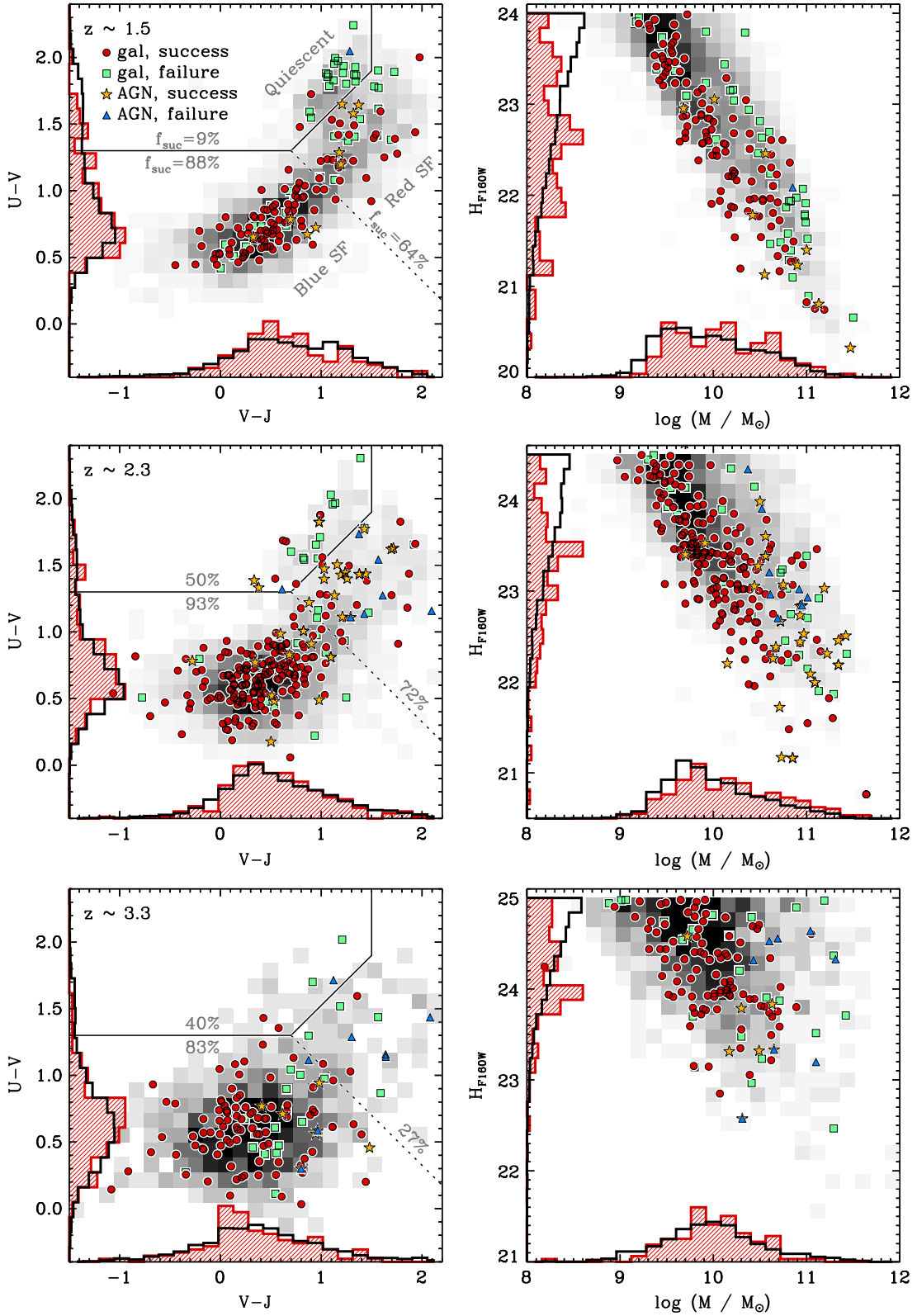
Figure 16. Left: rest-frame U-V vs. V-J color ( UVJ diagram) for the three different redshift intervals. Quiescent galaxies populate the sequence enclosed by the box in the top left of this diagram. Star-forming galaxies populate the bottom sequence. In gray scale we show the parent galaxy samples from which the targets are selected, with H -band magnitude limits of 24.0, 24.5, and 25.0, for the low-, middle-, and high-redshift intervals, respectively. The colored symbols represent our targeted objects, with red circles and yellow stars indicating galaxies and AGNs with robust spectroscopic redshifts. The green squares and blue triangles indicate targeted galaxies and AGNs for which no robust redshifts have been obtained. AGNs are identified by either their X-ray luminosity or IRAC colors (Coil et al. 2014). The success rate for quiescent galaxies, blue star-forming galaxies (below/to the left of the dotted line), and red star-forming galaxies (above/to the right of the dotted line) are given in gray. The open black and shaded red histograms represent the distribution of the parent and confirmed samples (galaxies and AGNs), respectively, for the property on the corresponding axis. The histograms are normalized to the same area. Right: H_{F160W} magnitude vs. stellar mass for the parent sample (gray scale) and the MOSDEF targeted galaxies and AGNs. Symbols and histograms are similar to those in the left panels.
