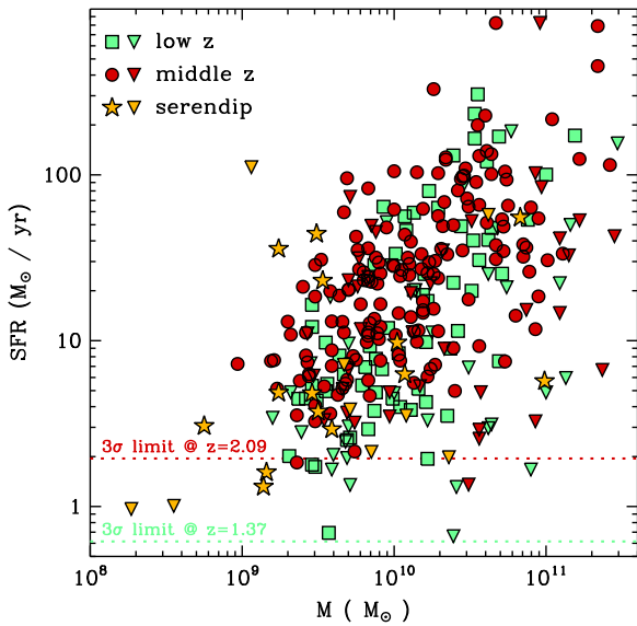
Figure 14. SFR vs. stellar mass for galaxies in the low (green) and middle redshift interval (red) for a Chabrier IMF. The 3\sigma upper limits are indicated by the upside-down triangles. The yellow symbols indicate the galaxies that were serendipitously detected. The SFRs are derived from the combination of H\alpha and H\beta . The 3\sigma limits on the SFR, calculated using the optimal 3\sigma line sensitivities in H and K, are shown for z \sim 1.37 and z \sim 2.09 (i.e., the lower boundaries of the redshift intervals), respectively. In this calculation we assume no dust attenuation.
