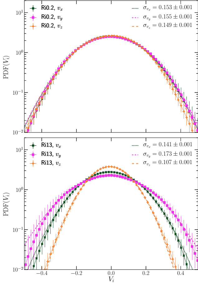
Figure 4. Time-averaged volume-weighted velocity-component PDFs with Gaussian fits for \text{Ri} = 0.2 (top) and \text{Ri} = 13 (bottom). The PDFs are Gaussian for all three components, but the velocity fluctuation is anisotropic for \text{Ri} \gtrsim 1 .
