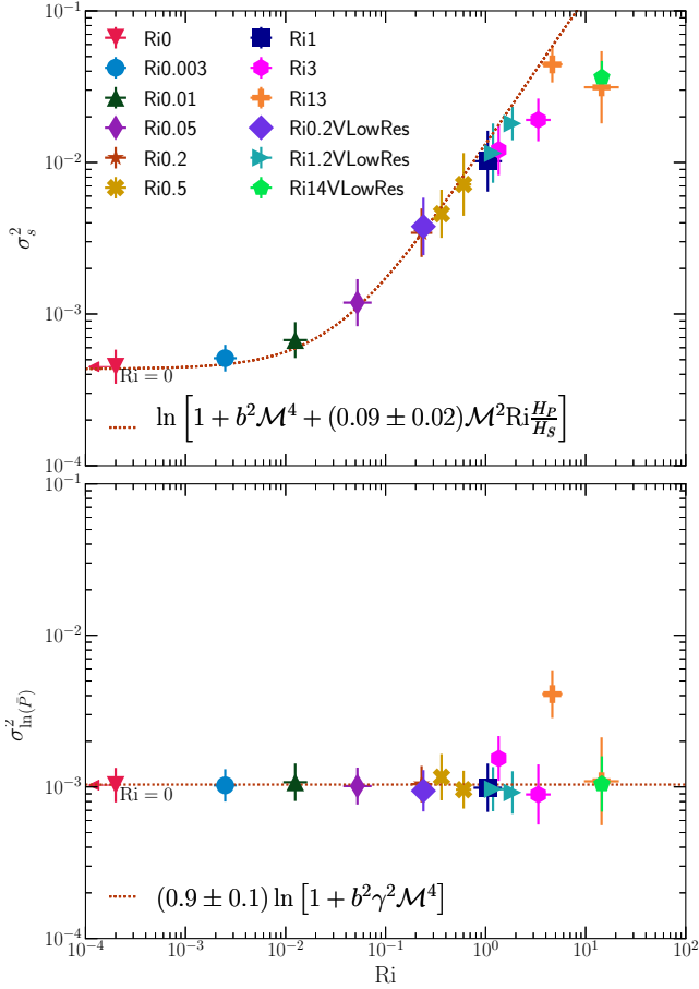
Figure 6. Upper panel: Scatter plot of \sigma_z versus Ri . The amplitude of density fluctuations increases as a function of Ri for 0.01 \lesssim Ri < 1 , reaches a peak at Ri \approx 10 and then starts decreasing for Ri > 10 . Lower panel: Scatter plot of \sigma_{\ln(\bar{p})} (defined in section 3.6) versus Ri . Pressure fluctuations are roughly independent of Ri . The outlier point has a larger local \mathcal{M} which makes it consistent with the baseline relation. Note: We conduct ‘VLowRes’ runs with resolution 256^2 \times 384 , but with different H_P/H_\rho (and thus different H_P/H_S ), with simulation parameters described in table 2. For these runs, we have plotted \sigma_{s, \text{scaled}} calculated using eq. (21) instead of \sigma_s .
