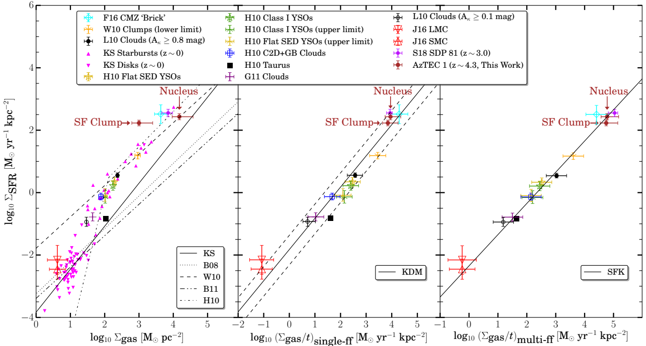
Figure 4. Comparison of star formation relations in multiple datasets, showing the measured and predicted SFRs, overlaid with the two regions of AzTEC-1 in brown. Asymmetric error bars for AzTEC-1 regions are a result of the systematic uncertainty on the CO excitation scale factor r_{43} . Left-panel: Measured SFR surface density as a function of the gas surface density (equation 1) in numerous star-forming regions (Heiderman et al. 2010 (H10), Lada et al. 2010 (L10), Wu et al. 2010 (W10), Gutermuth et al. 2011 (G11), Jameson et al. 2016 (J16), Federrath et al. 2016 (F16) and Sharda et al. 2018 (S18)). Also plotted are the SFR relations proposed by Bigiel et al. 2008 (B08), Bigiel et al. 2011 (B11), Wu et al. 2010 (W10) and Heiderman et al. 2010 (H10). Middle-panel: Measured SFR surface density plotted against the single-freefall time model by Krumholz et al. 2012 (equation 2). The dashed lines depict deviations by a factor of 3 from the best-fit relation (see also Krumholz et al. 2013). Right-panel: Measured SFR surface density plotted against the multi-freefall model of Salim et al. 2015 (equation 3).
