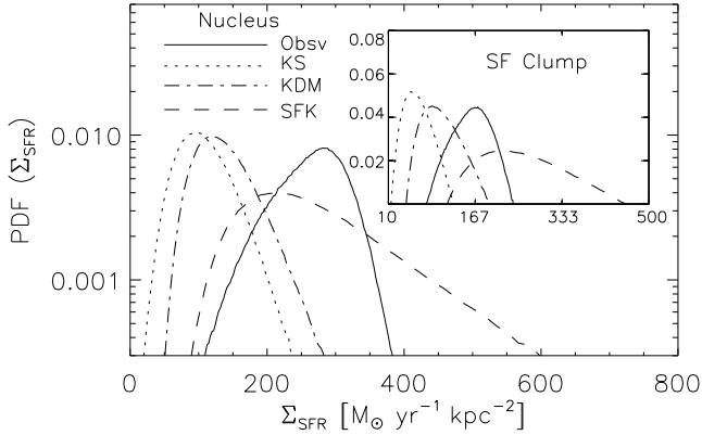
Figure 2. Probability distribution function (PDF) of the star formation rate (SFR) surface density ( \Sigma_{\text{SFR}} ) in the nucleus, estimated from the data and those predicted from KS (dotted curve, equation 1), KDM (dot-dashed curve, equation 2) and SFK (dashed curve, equation 3) relations. Inset depicts the same PDFs for the star-forming (SF) clump.
