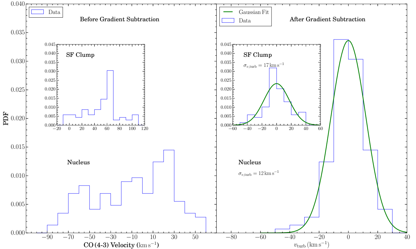
Figure 3. PDF of the CO (4-3) velocities (as labelled in Figure 1) and velocities after the subtraction of the local, linear velocity gradient ( v_{\text{turb}} ). The standard deviation ( \sigma_{v,\text{turb}} ) of the turbulent velocity (gas velocity after gradient subtraction) yields the turbulent Mach number ( \mathcal{M} ) in the two regions. Inset depicts the same for the star-forming (SF) clump.
