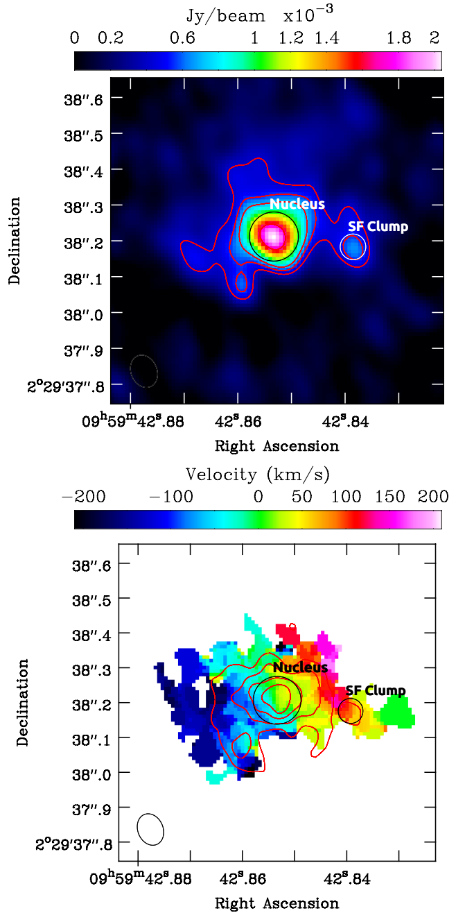
Figure 1. 0.093'' \times 0.072'' ( 624 \times 483 \text{ pc} ) resolution maps of \lambda_{\text{obs}} = 860 \mu\text{m} continuum flux density and CO (4-3) velocity in AzTEC-1 (beam size as depicted in the lower left corners). The white and black circles in the two panels depict the nucleus and the star-forming (SF) clump we analyze in this work. The red contours in the continuum map correspond to 5, 7, 9 and 21 \sigma_{860 \mu\text{m}} while those on the velocity map correspond to CO (4-3) velocity integrated flux density, plotted at 5, 7, 9 and 11 \sigma_{\text{CO}(4-3)} .
