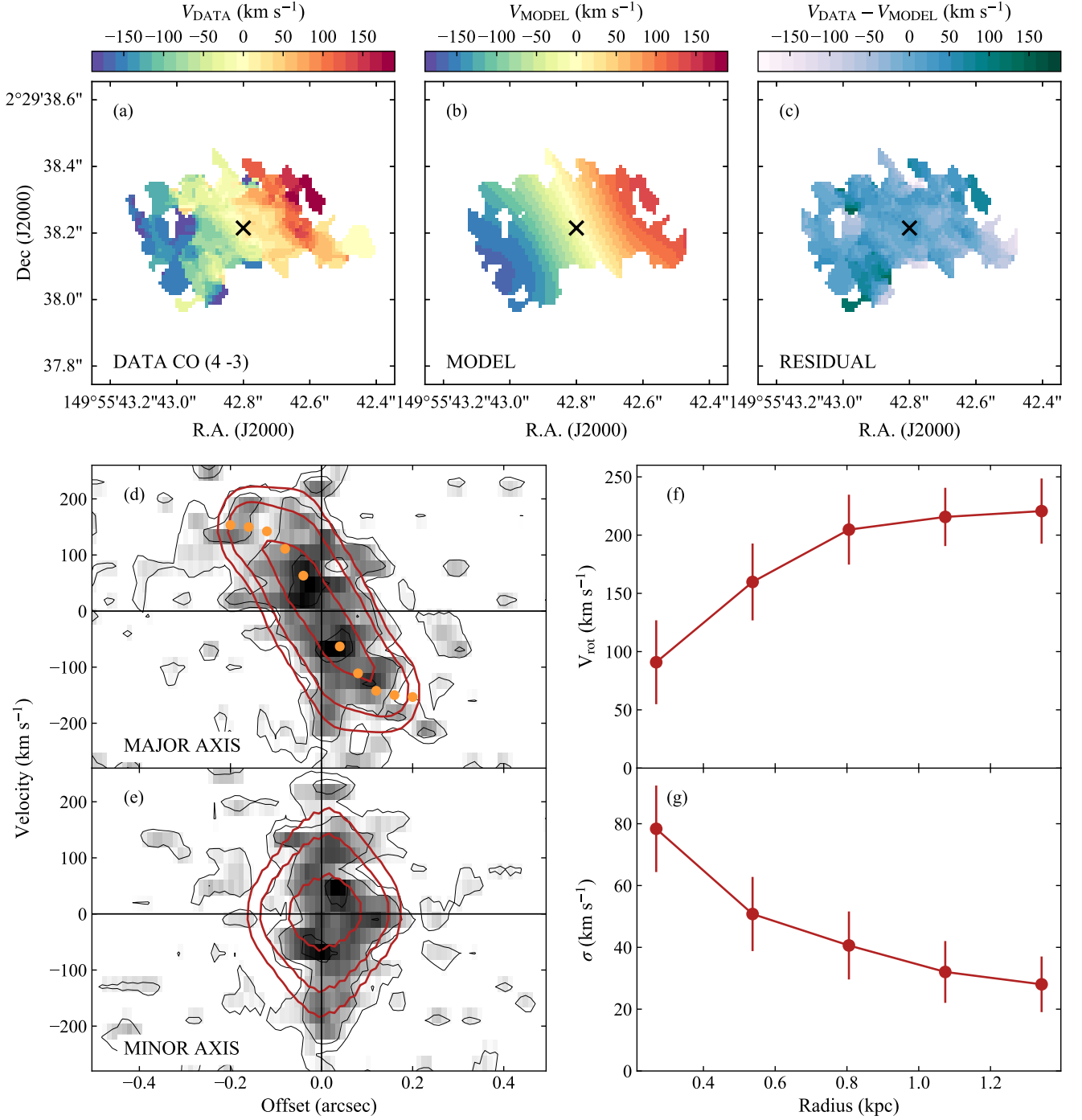
Figure A.1. Kinematic modelling of AzTEC-1 with 3^{\text{D}} BAROLO. Panels (a)-(b)-(c): observed velocity field (same as Figure 1), model velocity field and residuals (data-model). Black crosses represent the kinematic centre of the galaxy. Panels (d)-(e): position-velocity cuts taken along the major and minor axes of the galaxy. Data are shown in greyscale and black contours, model in red contours. Contour levels are at 1.5\sigma_{\text{RMS}} , 3\sigma_{\text{RMS}} and 5\sigma_{\text{RMS}} , with \sigma_{\text{RMS}} = 78 \mu\text{Jy} being the rms noise of the data. Orange dots in panel (d) denote the derived rotation velocity (not corrected for inclination). Panels (f)-(g): rotation curve and velocity dispersion profile along the line of sight.
