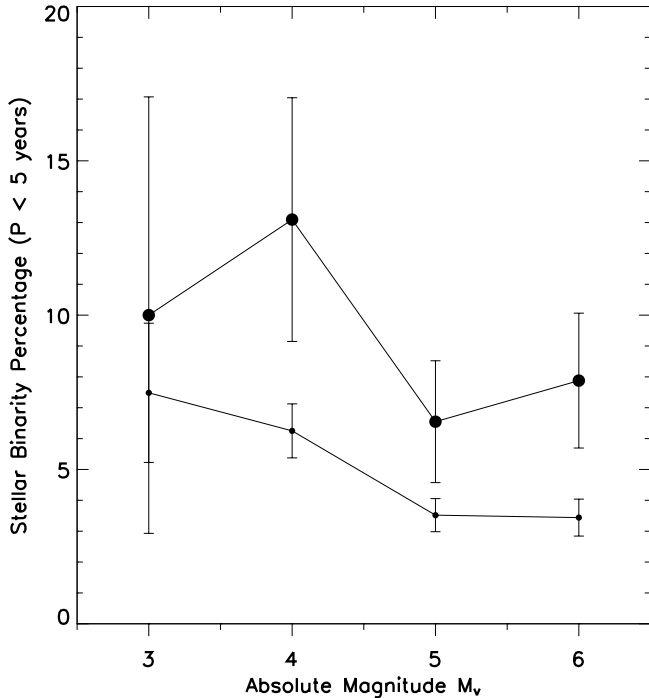
FIG. 3.—Fraction of stars that are known to be close ( P < 5 yr) Doppler binaries as a function of absolute magnitude. For the 25 pc Sun-like sample (large dots), \sim 11\% of stars are binaries; within the error bars, brighter stars do not appear to be significantly overrepresented. If we include the extra stars to make the 50 pc Sun-like sample (small dots), the stellar binary fraction is lower and decreases as the systems get fainter.
