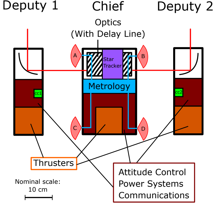
Figure 1. Schematic of the satellite array. The metrology system measures distances from optical heads A and C to corner cube 1 (cc1), and from optical heads B and D to corner cube 2 (cc2).
