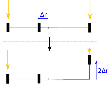
Figure 4. Potential routine for correcting for drag. In the top panel, drag has caused the chief to move a distance \Delta r from the centre of the array. To correct for this, we could boost the deputy with the longer separation up 2\Delta r in the direction of the star. Essentially, compensating an increase in |\Delta \mathbf{r}| with an increase in \Delta \mathbf{r} \cdot \hat{s} , so that D is kept close to 0 (see Equation 1).
