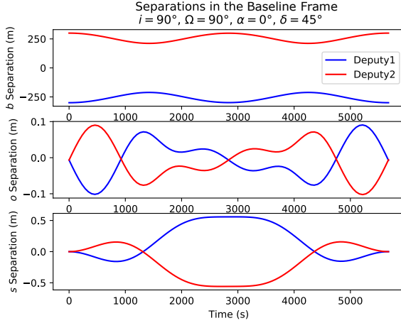
Figure 3. ECI integrated J_2 perturbed motion of the two deputy spacecraft with respect to the chief spacecraft over 1 orbit, with a chief orbital configuration of i = 90^\circ , \Omega = 90^\circ , and star coordinates \alpha = 0^\circ , \delta = 45^\circ
