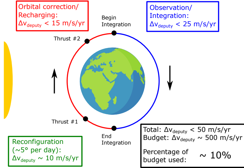
Figure 5. Summary of the \Delta v required by a deputy satellite to correct for orbital perturbations over a year.
