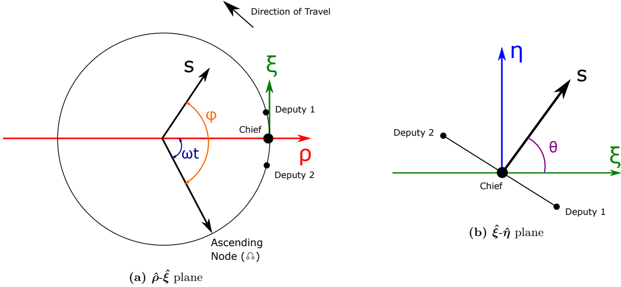
Figure 2. Schematic of the LVLH frame, including the star vector angles \theta and \phi .
