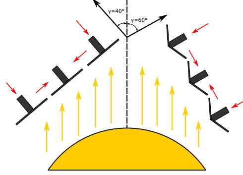
Figure 6. Schematic of keeping the satellite array within 40/60^\circ of the antisolar axis. Note that the solar panels can be used to baffle the sun, even for high antisolar angles \gamma , by folding them inwards slightly.
