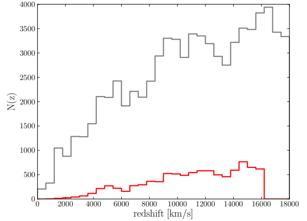
Figure 4. Redshift distribution of the 6dFGSv FP sample (red; N_g=8901 ) with maximum redshift cz_{max}=16120 \text{ km s}^{-1} compared to the full 6dFGS redshift sample (grey; N_g=124646 ).
