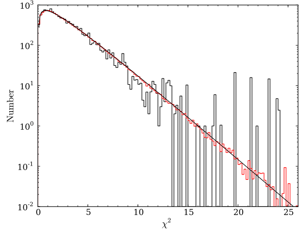
Figure 5. The distribution of \chi^2 for the galaxies in the observed J band FP sample (black) and for mock galaxies in a sample drawn from the best-fitting 3D Gaussian model (red). The smooth curve is an analytic \chi^2 distribution with 2.65 degrees of freedom, derived by fitting to the mock sample (there are fewer than 3 degrees of freedom due to the censoring of the 3D Gaussian by selection effects).
