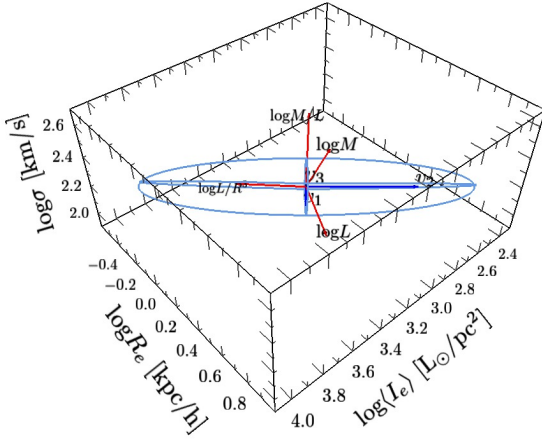
Figure 3. An interactive 3D schematic of FP space, showing the vectors \mathbf{v}_1, \mathbf{v}_2, \mathbf{v}_3 (in dark blue) that define the axes (see equation 5) of our Gaussian model ( 3\sigma Gaussian ellipsoid in cyan) as they are oriented with respect to the three observational parameter axes \mathbf{r}, \mathbf{s}, \mathbf{i} . We also show (in red) the vectors corresponding to the physical quantities \log M/L , \log M , \log L/R^3 as defined in §2.3. We note that the angle between the vectors \log M/L and -\mathbf{v}_1 and also \log L/R^3 and -\mathbf{v}_1 are both within 5^\circ of each other. (Readers using Acrobat Reader v8.0 or higher can enable interactive 3D viewing of this schematic by mouse clicking on the figure; see Appendix B for more detailed usage instructions.)
