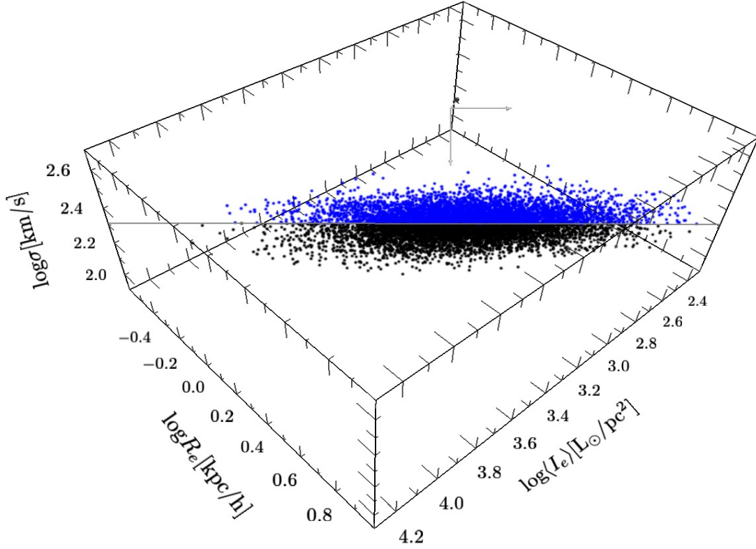
Figure 9. Interactive 3D visualisation of the 6dFGS J band Fundamental Plane in r, s, i space. The best fitting plane (in grey) has slopes a = 1.523 and b = -0.885 , and an offset c = -0.330 . The galaxies are colour-coded according to whether they are above (blue) or below (black) the best-fit plane. The 1\sigma , 2\sigma , and 3\sigma contours of the 3D Gaussian distribution (light grey) can be toggled in the interactive plot environment. (Readers using Acrobat Reader v8.0 or higher can enable interactive 3D viewing of this schematic by mouse clicking on the figure; see Appendix B for more detailed usage instructions.)
