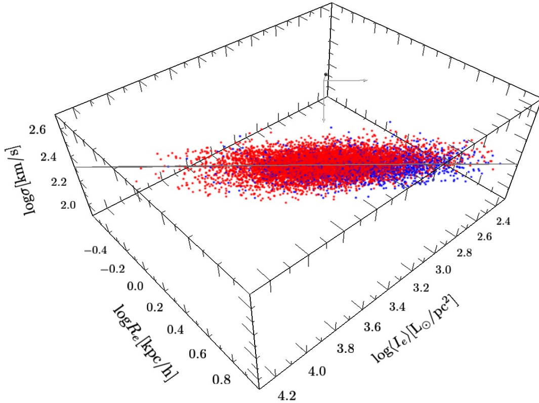
Figure 17. Interactive 3D visualisation of the 6dFGS J band Fundamental Plane in (r, s, i) -space. The best-fitting plane (in grey) for the J band (with a = 1.523 , b = -0.885 and c = -0.330 ) is plotted for reference. The galaxies are colour-coded according to morphology: 6956 early types in red and 1945 late types in blue. (Readers using Acrobat Reader v8.0 or higher can enable interactive 3D viewing of this schematic by mouse clicking on the figure; see Appendix B for more detailed usage instructions.)
