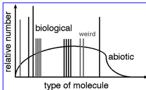
FIG. 2. Comparison of biogenic with nonbiogenic distributions of organic material. Nonbiological processes produce smooth distributions of organic material, illustrated here by the curve. Biology, in contrast, selects and uses only a few distinct molecules, shown here as spikes ( e.g. , the 20 L-amino acids used by familiar life).
