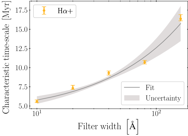
Figure 7. Characteristic emission time-scales for H\alpha + filters as a function of the filter width. The grey curve shows the fit described in equation (9) and the shaded region indicates the associated uncertainty.
