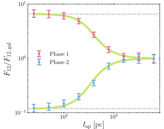
Figure 1. Example tuning fork diagram produced by the HEISENBERG code. The figure shows the relative change of the phase-1-to-phase-2 flux ratio ( F_{12} ) when placing apertures of size l_{ap} at the locations of emission peaks in the phase 1 map (top branch, in red) or the phase 2 map (bottom branch, in blue), compared to the galactic-scale phase-1-to-phase-2 flux ratio ( F_{12,gal} ) as a function l_{ap} . The best-fitting model is indicated by the two green curves.
