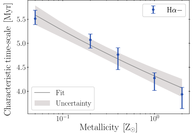
Figure 8. The relation between metallicity and characteristic time-scale for a well-sampled IMF for H\alpha - filters. The grey curve gives the fits described by equation (10). The shaded region indicates the associated uncertainty.
