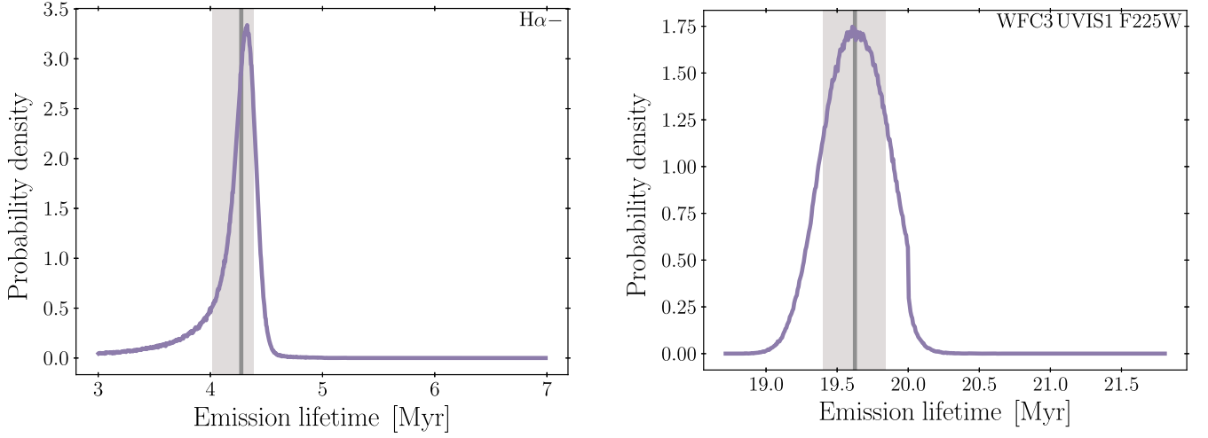
Figure 5. Two examples showing the PDFs associated with the defined characteristic time-scales. Left: H \alpha emission excluding the continuum (H \alpha -). Right: UV emission (WFC3 UVIS1 F225W). The vertical line shows the selected time-scale (the median of the distribution); the shaded region, the uncertainty defined by the 16th and 84th percentiles.
