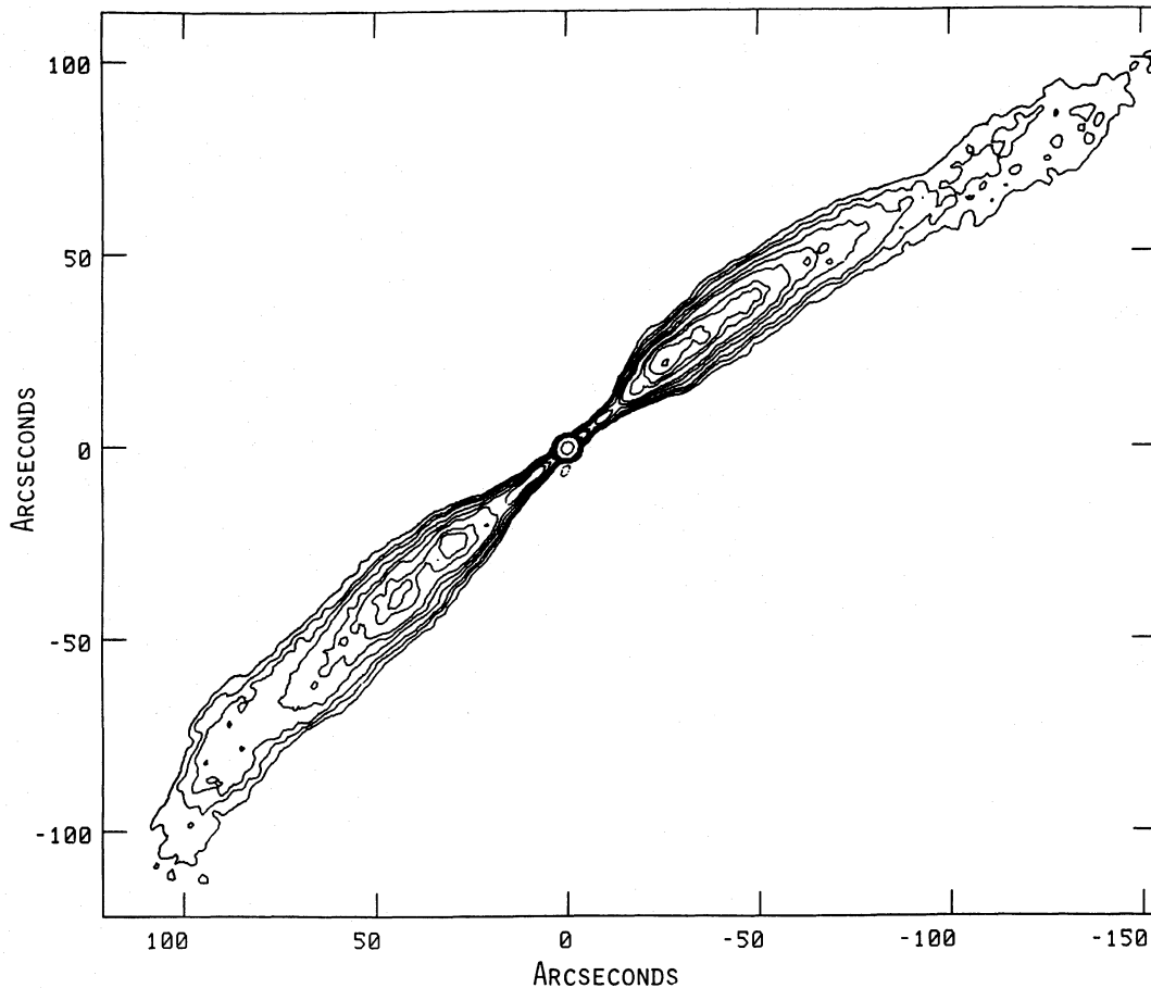
FIG. 10.—Jets at 20 cm with a 3''.2 FWHM beam made from the B + A_n -configuration data set only. Peak flux is 153.1 mJy per beam, and the contour levels are -1\% , 1\% , 1.5\% , 2\% , 3\% , 4\% , 5\% , 7\% , 8\% , 9.5\% , 11.5\% , and 50\% of the peak. Noise in the map is approximately 0.25 mJy per beam.
