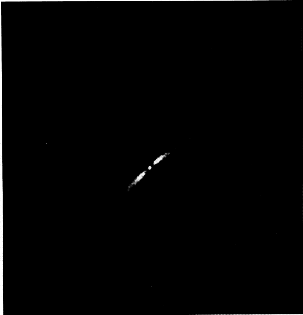
FIG. 9.—Radiograph of the jets at 20 cm with 10'4 resolution
