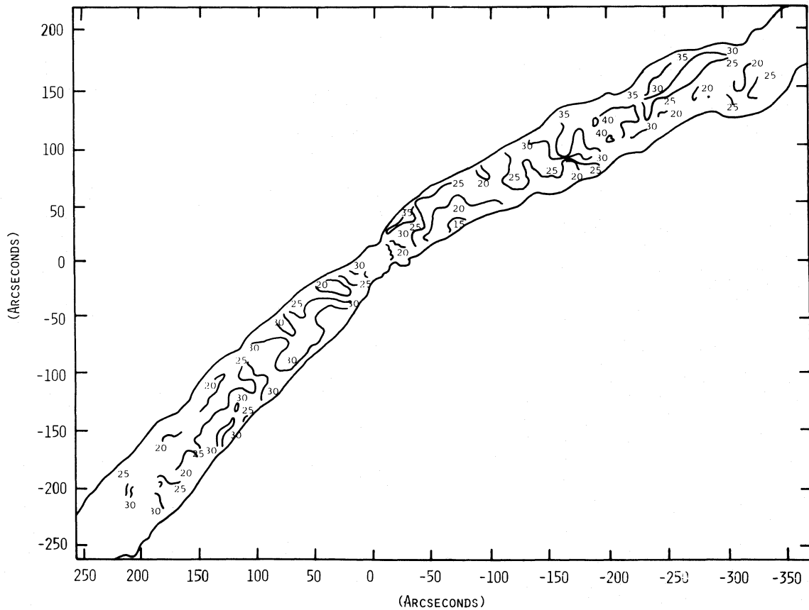
FIG. 22.—Schematic contour diagram of -1 times the 6–20 cm rotation measure ( \text{rad m}^{-2} ) at 10'' resolution. Outer contour is at the total intensity, 20 cm, 10'' resolution, 1% of peak level (see Fig. 8).
