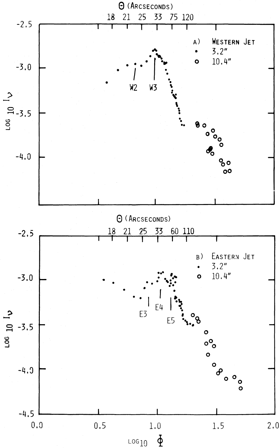
FIG. 18.— \log_{10} of the deconvolved 20 cm ridge line surface brightness, I_{\nu} ( \text{mJy arcsec}^{-2} ), plotted against \log_{10} of the deconvolved jet FWHM, \Phi (arcsec), for both jets—(a) is west; (b) is east. The 3.2" resolution data are used for \Theta < 120'' , while for \Theta > 120'' the 10.4" resolution data are shown. Upper horizontal axis gives an approximate scale in \Theta ( \Theta < 120'' ) since \Theta is generally monotonic in that region.
