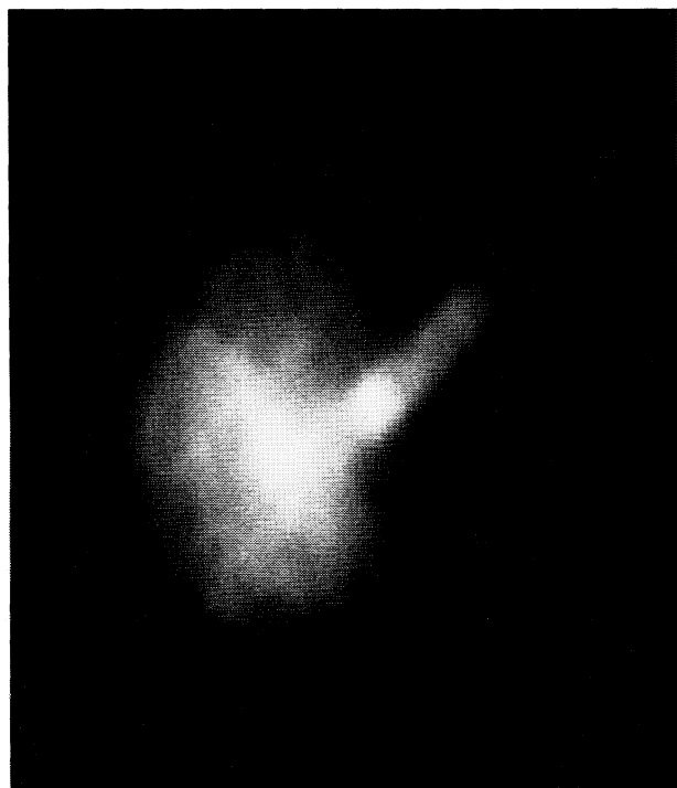
FIG. 5.—Radiograph of the eastern lobe at 6 cm with 26'' resolution. This image has not been primary beam corrected for display purposes only. However, the primary beam correction is substantial at the eastern edge of the lobe (the field center is close to the knot where the jet and lobe merge).
