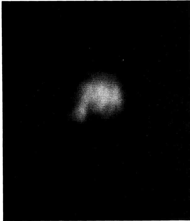
FIG. 7.—Radiograph of the western lobe at 6 cm with 26" resolution. This image has not been primary beam corrected for display purposes only. However, the primary beam correction is substantial at the edges of the lobe.
