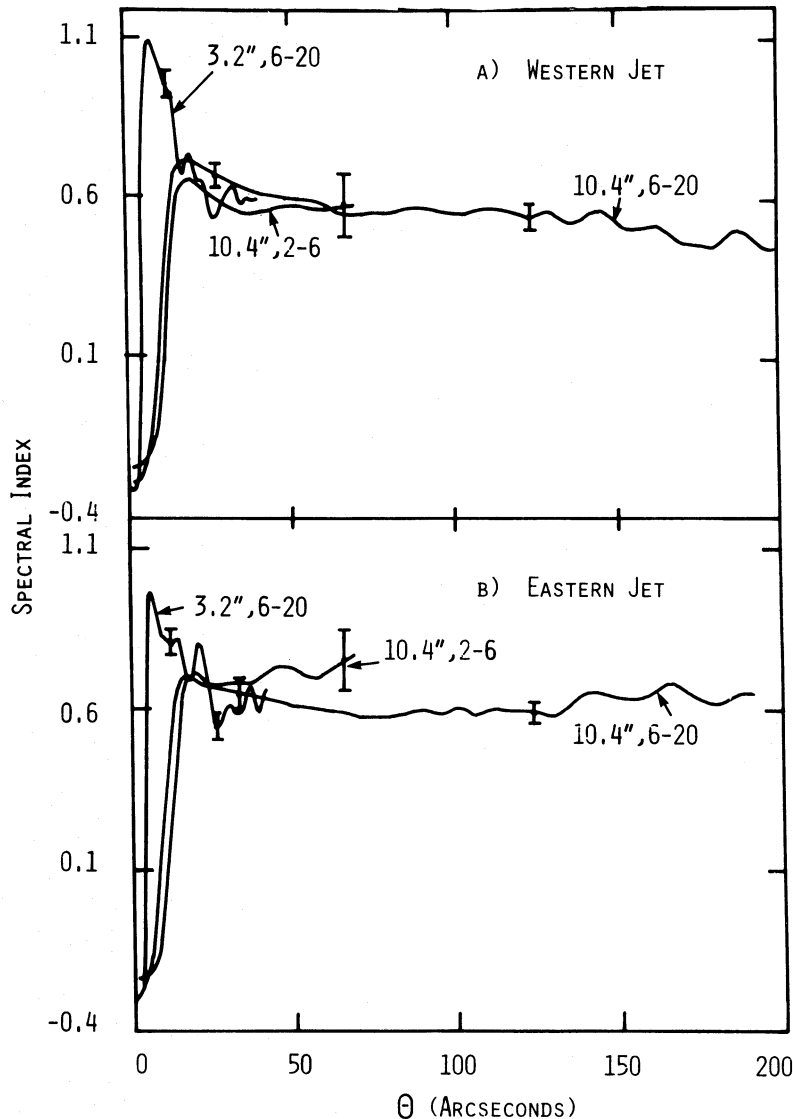
FIG. 20.—The 6–20 cm (3''/2 and 10''/4 resolution) and the 2–6 cm (10''/4 resolution) spectral index as a function of angular distance from the core, \Theta (arcsec), for both jets: (a) is west; (b) is east. Bars indicate approximate errors due to noise.
