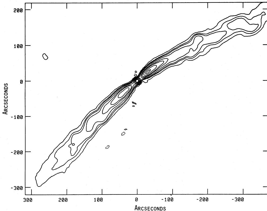
FIG. 8.—Jets at 20 cm with a 10".4 FWHM beam made from the C-, C + A n -, and B + A n -configuration data sets. Peak flux is 163.1 mJy per beam, and the contour levels are -3%, -1%, 1%, 3%, 5%, 10%, 20%, 30%, 50%, and 70%, of the peak. Noise in the map is approximately 0.3 mJy per beam.
