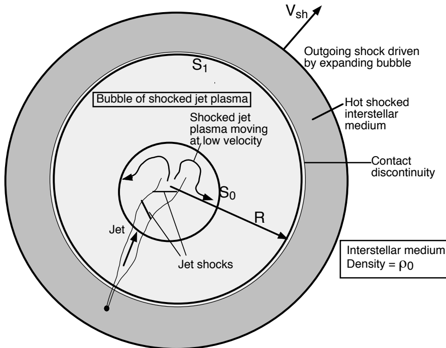
Fig. 2.— Schematic of a jet-inflated bubble.
