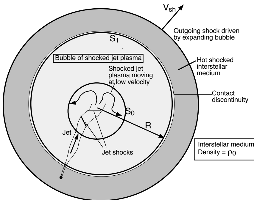
Fig. 2.— Schematic of a jet-inflated bubble.
