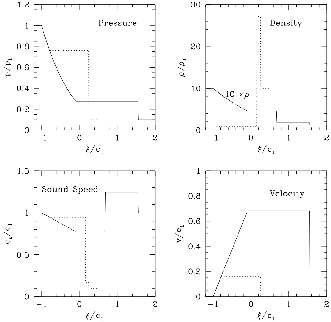
Fig. 1.— The pressure, density, sound speed and velocity in a shock tube.
