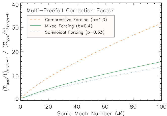
Figure 1. The multi-freefall correction factor derived in Equation (9) as a function of the sonic Mach number for three values of the turbulent driving parameter b whilst neglecting magnetic fields ( \beta \rightarrow \infty ). The values in the figure represent the correction factor are applied to existing measurements of (\Sigma_{\text{gas}}/t)_{\text{single-ff}} in order to correct them to (\Sigma_{\text{gas}}/t)_{\text{multi-ff}} .
