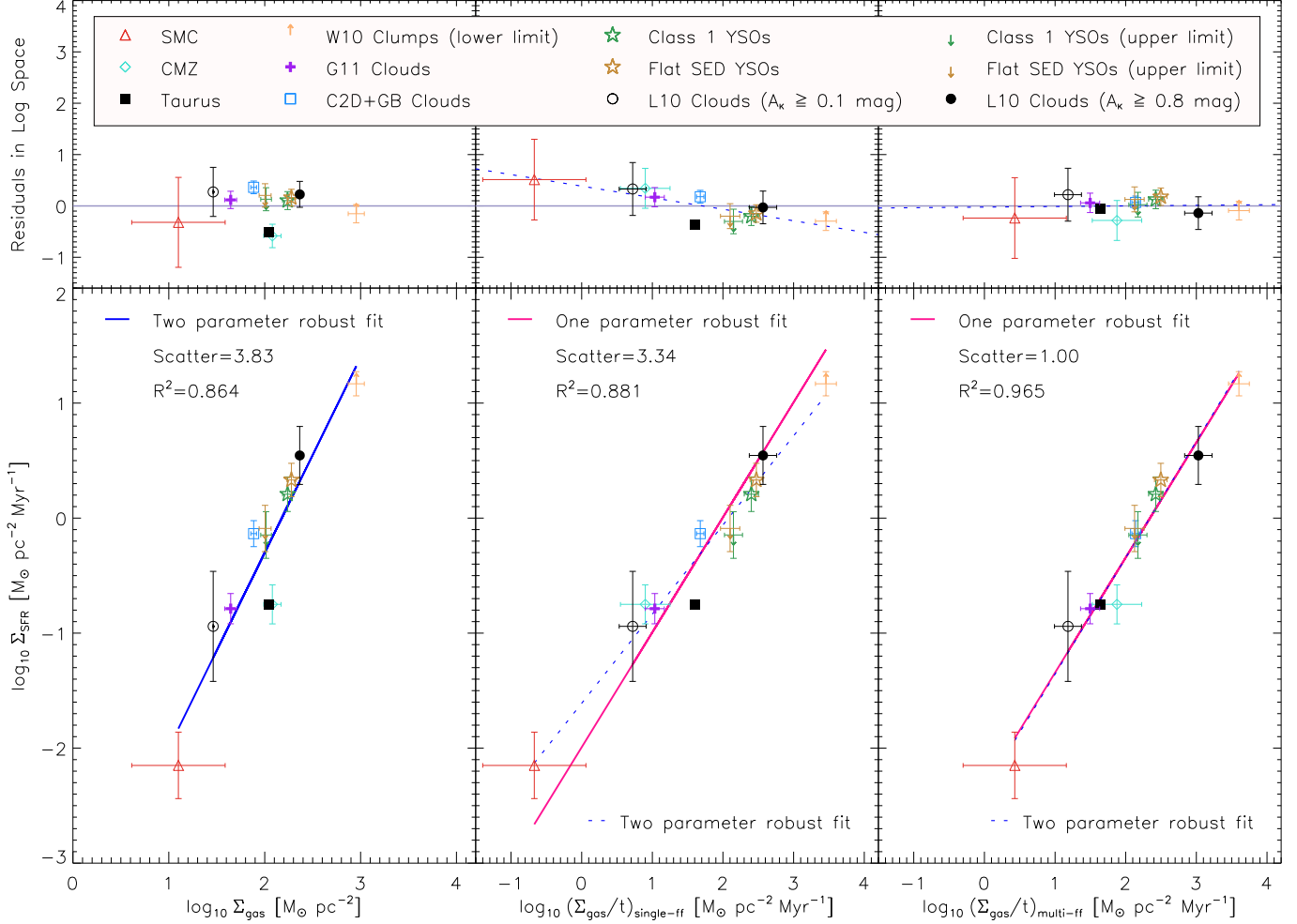
Figure 2. Bottom panels: \Sigma_{\text{SFR}} versus \Sigma_{\text{gas}} (classical Kennicutt-Schmidt relation; left), \Sigma_{\text{SFR}} versus (\Sigma_{\text{gas}}/t)_{\text{single-ff}} (Krumholz et al. 2012, middle), and our new model, \Sigma_{\text{SFR}} versus (\Sigma_{\text{gas}}/t)_{\text{multi-ff}} (right) for the observational data in Table 1. Power-law fits are shown as solid lines and the respective goodness-of-fit parameter R^2 (where R^2 = 1 corresponds to a perfect fit) is shown in each panel, as well as the normalized scatter. We also apply a two-parameter robust line fit to these relations, shown as the dotted lines. We find that our new multi-freefall SF law provides the best correlation with a reduced scatter by a factor of 3–4 compared to the previous SF laws. Top panels: The residuals of each relation in log space versus each of the parameterizations being analyzed. The solid and dotted lines in each panel are respectively the fits shown in the bottom panels.
