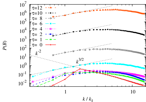
FIG. 4.— Time evolution of the magnetic field spectra for the run with 128 cells per Jeans length as a function of wavenumber, normalized to the local Jeans wavenumber, i.e., the magnetic field inside the dense core is shown for each timestep, in the collapsing frame of reference. The initial magnetic field spectrum ( \tau = 0 ) follows the initial power law, P(B) \propto k^{-2} on scales smaller than the peak scale at k/k_J \approx 1.4 . Within the regime of turbulent decay ( 0 < \tau < 4 ), the peak shifts to k/k_J \approx 5-6 due to dynamo amplification, which is most efficient on small scales (discussed further in section 4.1). The magnetic field spectra are consistent with the generic k^{3/2} Kazantsev spectrum (Kazantsev 1968; Brandenburg & Subramanian 2005) on scales smaller than the Jeans length and larger than the peak. Within the collapse regime, the magnetic energy grows exponentially on all scales within the core.
