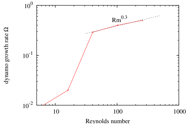
FIG. 10.— Dynamo growth rate, \Omega , measured in Fig. 9 as a function of Reynolds number. Note the strong increase in the growth rate for \text{Rm} \lesssim 40 , which corresponds to a Jeans resolution of about 30 grid cells.
