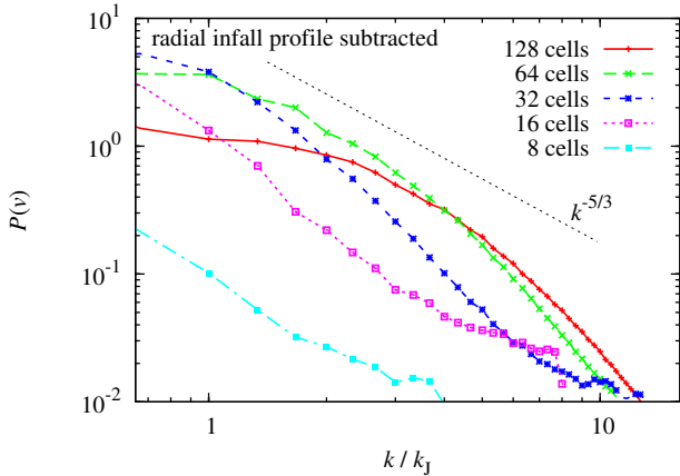
FIG. 11.— Shows the resolution dependence of the velocity spectra at \tau = 12 . The spectra do not show convergence, even with a Jeans resolution of 128 cells. We expect that a resolution of 512^3 grid cells inside the Jeans volume is required to obtain an inertial range. The expected Kolmogorov (1941) scaling of the turbulence in the inertial range is shown only for comparison. The total turbulent energy, i.e., the integral over the spectra, however, indicates convergence for a Jeans resolution of 32 cells and more (see Fig. 12).
