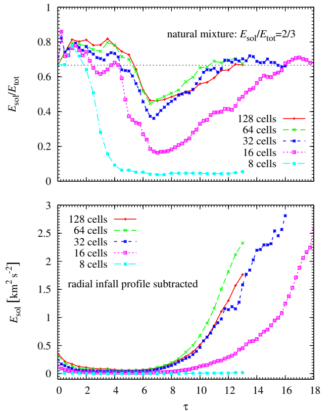
FIG. 12.— Top: time evolution of the solenoidal ratio, \chi = E_{\text{sol}}/E_{\text{tot}} , eq. (12), for Jeans resolutions of 8, 16, 32, 64, and 128 grid cells. Bottom: Turbulent energy in solenoidal modes for the infall-subtracted motions inside the core. The runs with 32, 64, and 128 cells indicate convergence of \chi (top panel) and in the absolute rotational energy, E_{\text{sol}} (bottom panel), while the 8 and 16 cell runs clearly underestimate the amount of rotational energy.
