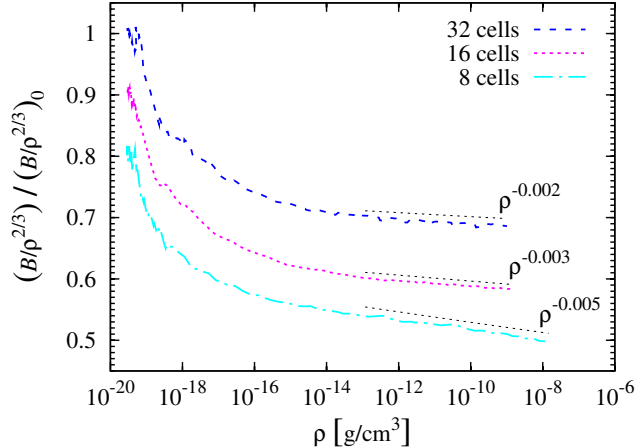
FIG. 13.— Test on the numerical diffusion of the magnetic field in the HLL3R scheme for ideal MHD (Waagan et al. 2011). Three runs with Jeans resolutions of 8, 16, and 32 cells are shown. For clarity, the curves for 16 and 8 cells were shifted down by 10 and 20%, respectively. The initial decrease of B/\rho^{2/3} is due to the anisotropic geometry of the initial field structure. At late times during the collapse, the field becomes approximately isotropic due to the bending of the field lines to an hour-glass shape. In this regime, we can estimate upper limits for the effects of numerical diffusion, indicated by the dashed lines for \rho > 10^{-13} \text{ g cm}^{-3} .
