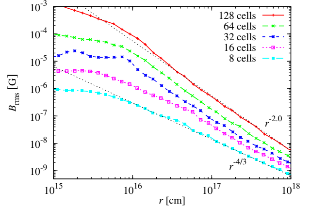
FIG. 2.— Power-law part of the radial profiles of the rms magnetic field at \tau = 12 for Jeans resolutions of 8, 16, 32, 64, and 128 cells. Power laws corresponding to pure flux-freezing, B_{\text{rms}} \propto r^{-4/3} , and a steeper, \propto r^{-2.0} profile are drawn for comparison.
