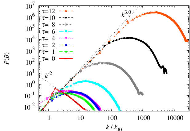
FIG. 5.— Magnetic energy spectra in the fixed frame of reference, i.e., the spectra are normalized to the initial Jeans wavenumber, k_{J0} . The time evolution in the collapse regime shows that the magnetic field is basically frozen-in on large scales, while the turbulent dynamo keeps amplifying the field on smaller and smaller scales as the collapse proceeds.
