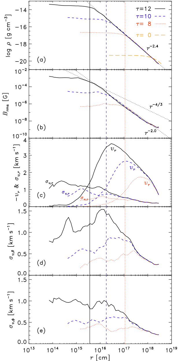
FIG. 1.— a) Radial density profile of the collapsing, magnetized, turbulent Bonnor-Ebert sphere at times \tau = 8, 10, and 12 . b) Same as a) but for the rms magnetic field. c) Same as a) but for the infall velocity, -v_r and the radial velocity dispersion, \sigma_{v,r} . d) and e) Same as a) but for the polar and azimuthal velocity dispersions, \sigma_{v,\theta} and \sigma_{v,\phi} . The vertical lines extending through all panels indicate the Jeans radius at \tau = 8, 10, and 12 , respectively. See paper I for the corresponding radial profiles of the rms velocity and Mach number.
