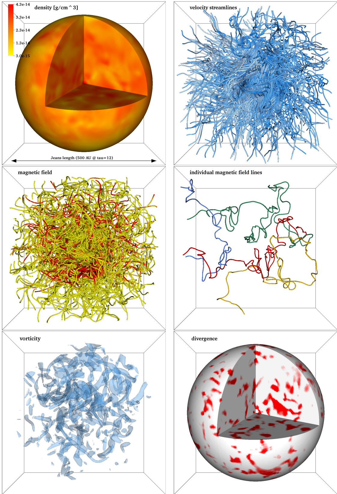
FIG. 3.— a) Spherical slice of the gas density inside the Jeans volume at \tau = 12 for our run with 128 cells per Jeans length. b) Velocity streamlines on a linear color scale ranging from dark blue ( 0 \text{ km s}^{-1} ) to light gray ( 5 \text{ km s}^{-1} ). c) Magnetic field lines, showing a highly tangled and twisted magnetic field structure typical of the small-scale dynamo; yellow: 0.5 \text{ mG} , red: 1 \text{ mG} . d) Four randomly chosen, individual field lines. The green one, in particular, is extremely tangled close to the center of the Jeans volume. e) Contours of the vorticity modulus, |\nabla \times \mathbf{v}| , showing elongated, filamentary structures typically seen in subsonic turbulence (e.g., Frisch 1995). f) Spherical slice of the divergence of the velocity field, \nabla \cdot \mathbf{v} ; white: compression, red: expansion.
