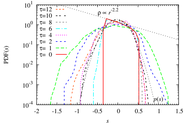
FIG. 6.— Time evolution of the probability distribution functions (PDFs) of the logarithmic gas density, s \equiv \ln(\rho/\langle\rho\rangle) , inside the collapsing core. The initial density PDF is characterized by the asymptotic radial profile of a Bonnor-Ebert sphere at low densities, \rho \propto r^{-2.2} , while at higher densities, it turns into a steeper PDF due to the flat inner core. The PDFs in the turbulent decay regime ( \tau \lesssim 4 ) are convolutions of the PDF of the initial density distribution and log-normal distributions typical of turbulence. In the collapse regime ( \tau \gtrsim 4 ), the PDFs are close to log-normal distributions, with some modification due to the radial density distribution (see Fig. 1). The dotted curve shows a log-normal fit using equation (7) with the imposed condition, eq. (8) at \tau = 10 .
