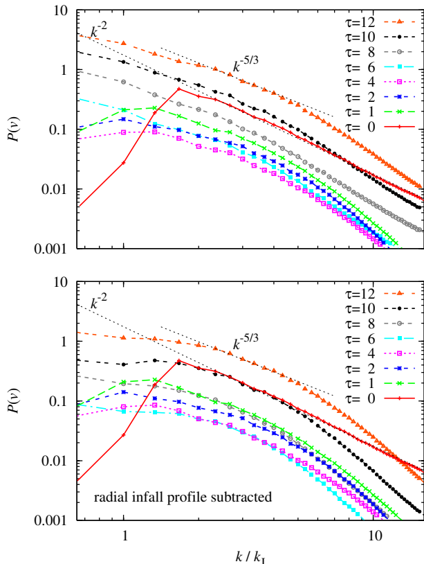
FIG. 7.— Top: Velocity power spectra normalized to the local Jeans wavenumber, k/k_J , inside the core for different times until \tau = 12 . Bottom: same as top, but for the infall-subtracted velocity spectra. The flattening of the infall-subtracted spectra around k/k_J \approx 1-2 indicates that gravity-driven turbulence exhibits an effective driving scale close to the Jeans scale.
