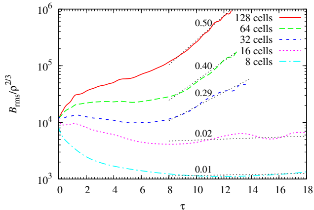
FIG. 9.— Shows the time evolution of the rms magnetic field strength as a function of Jeans resolution, where we divided out the effect of pure flux freezing, which can provide a maximum possible field amplification by \rho^{2/3} inside the core. The remaining amplification is thus due to the small-scale dynamo. The number on each curve indicates the growth rate, \Omega , in the expression B_{\text{rms}}/\rho^{2/3} \propto \exp(\Omega\tau) , measured in the interval \tau = [8, \tau_{\text{end}}] .
