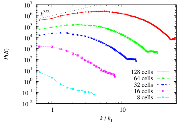
FIG. 8.— Shows the resolution dependence of the magnetic field spectra at \tau = 12 . The peak of the magnetic energy shifts to smaller scales for increasing Jeans resolution (32, 64, and 128 cells), but is completely absent for a Jeans resolution of 16 cells and below. We conclude that turbulent dynamo amplification of the magnetic field is only obtained, if the Jeans length is resolved with at least 30 grid cells.
