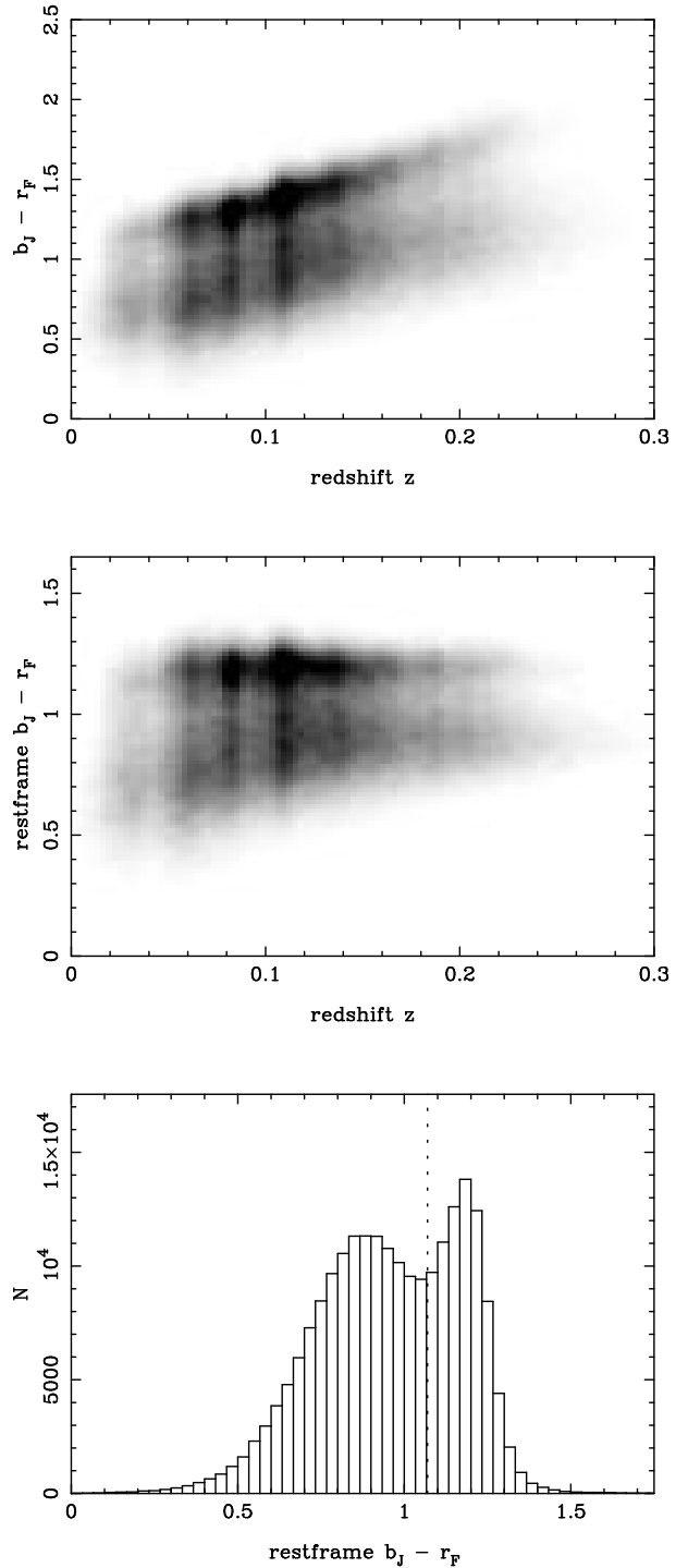
Figure 2. Photographic b_J - r_F colour versus redshift for the 2dFGRS, as observed and in the rest frame. The separation between ‘early-type’ (red) and ‘late-type’ (blue) galaxies is very clear. The third panel shows the histogram of k -corrected restframe colours, which is very clearly bimodal. This is strongly reminiscent of the distribution of the spectral type, \eta , and we assume that a division at (b_J - r_F)_0 = 1.07 (dotted line) achieves a separation of early-type ‘class 1’ galaxies from classes 2–4, as was done using spectra by Madgwick et al. (2002).
