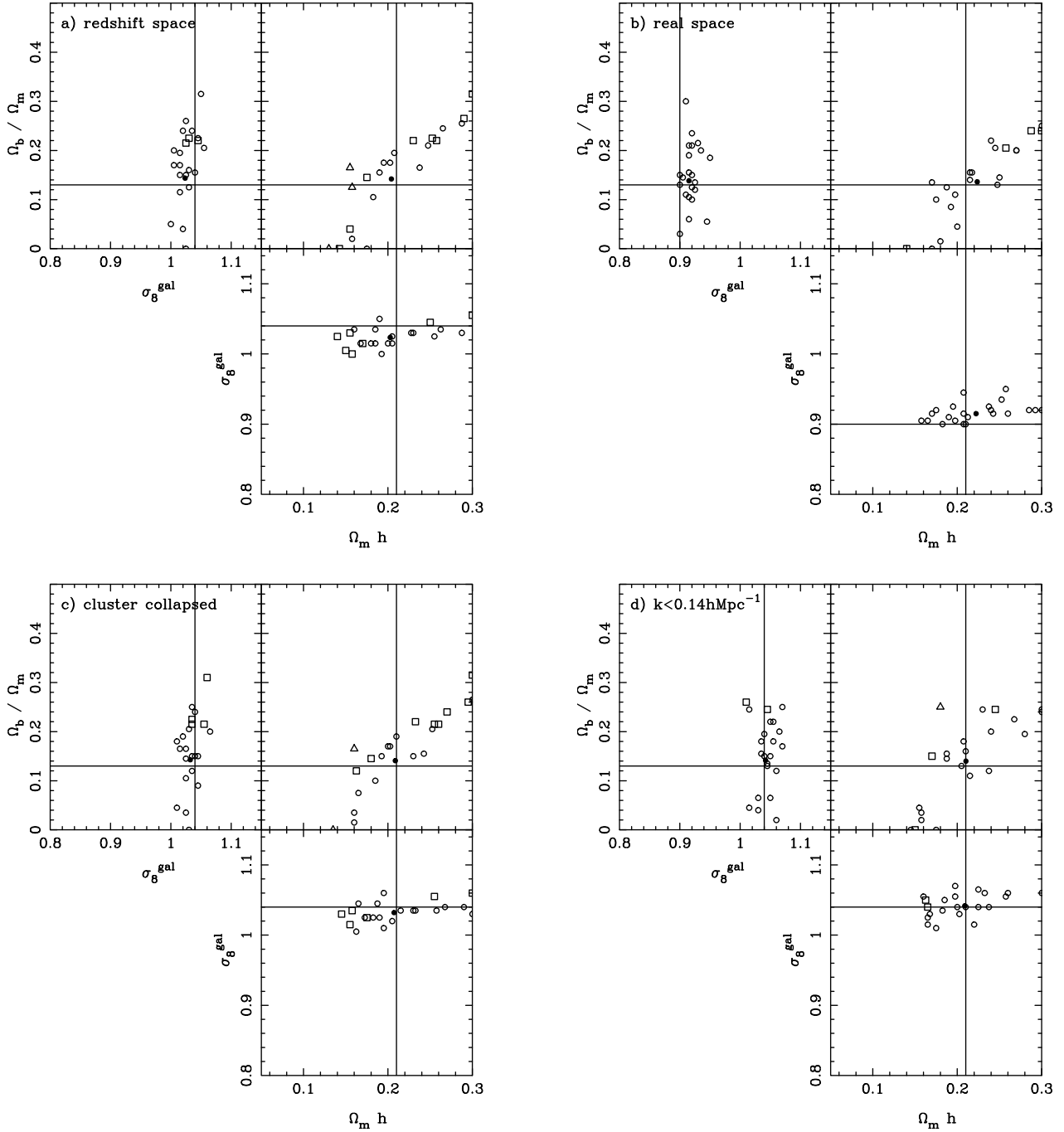
Figure 25. Recovered marginalized parameters from the Hubble Volume mock catalogues. The solid lines mark the true cosmological parameters and normalization of the Hubble Volume simulation, calculated from a large realization of galaxies covering the full Hubble Volume cube. Open circles mark the marginalized parameters recovered from mocks with 2(\ln \mathcal{L}_{\max} - \ln \mathcal{L}_{\text{true}}) < 2.3 (corresponding to mocks with recovered parameters less than 1\sigma from the true values), open squares 2.3 < 2(\ln \mathcal{L}_{\max} - \ln \mathcal{L}_{\text{true}}) < 6.0 ( 1\sigma to 2\sigma from the true values), and open triangles 2(\ln \mathcal{L}_{\max} - \ln \mathcal{L}_{\text{true}}) > 6.0 ( >2\sigma from the true values). The solid circle marks the average recovered parameters from all of the mocks. a) for the redshift-space Hubble Volume mocks fitting to 0.02 < k < 0.20 h \text{ Mpc}^{-1} marginalizing over Q . b) for the real-space Hubble Volume mocks. c) for the cluster-collapsed redshift-space mocks. d) for the redshift-space Hubble Volume mocks fitting to 0.02 < k < 0.14 h \text{ Mpc}^{-1} with Q = 0 .
