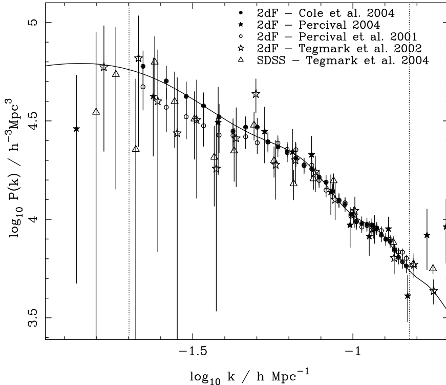
Figure 16. The redshift-space power spectrum calculated in this paper (solid circles) compared with other measurements of the 2dFGRS power spectrum shape by Percival et al. (2001) – open circles, Percival (2004c) – solid stars, and Tegmark et al. (2002) – open stars. For the data with window functions, the effect of the window has been approximately corrected by multiplying by the net effect of the window on a model power spectrum with \Omega_m h = 0.168 , \Omega_b/\Omega_m = 0.0 , h = 0.72 & n_s = 1 . A zero-baryon model was chosen in order to avoid adding features into the power spectrum. All of the data are renormalized to match the new measurements. The open triangles show the uncorrelated SDSS real space P(k) of Tegmark et al. (2004), calculated using their ‘modelling method’ with no FOG compression (their Table 3). These data have been corrected for the SDSS window as described above for the 2dFGRS data. The solid line shows a model linear power spectrum with \Omega_m h = 0.168 , \Omega_b/\Omega_m = 0.17 , h = 0.72 , n_s = 1 and normalization matched to the 2dFGRS power spectrum.
