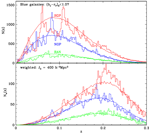
Figure 8. As Fig. 6 but for the blue subset with rest frame colours bluer than (b_J - r_F)_0 < 1.07 .
