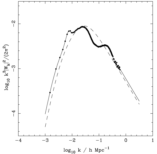
Figure 9. The amplitude of the spherically averaged 2dFGRS window function in Fourier space (filled circles). The solid line gives a cubic spline (Press et al. 1992) fit to these data and was used to perform the spherical convolution of model power spectra. For comparison, we also plot the fit used in Percival et al. (2001; P01), which ignores the structure in the window for k > 0.02 h \text{Mpc}^{-1} (dashed line).
