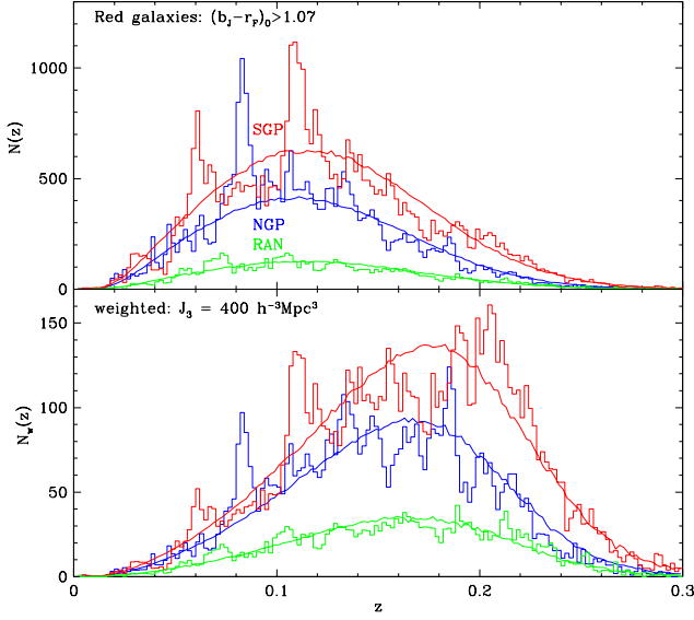
Figure 7. As Fig. 6 but for the red subset with rest frame colours redder than (b_J - r_F)_0 > 1.07 .
