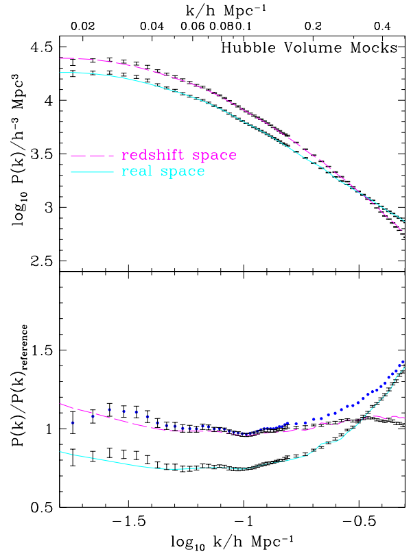
Figure 11. Comparison of the expected and recovered power spectra for the Hubble Volume mock catalogues. For mocks constructed using both real-space and redshift-space galaxies positions, we compare the input non-linear power spectrum (curves) with the mean recovered power spectrum (error bars). Unlike Fig. 10, the error bars here indicate the error in the mean recovered power, computed assuming the 22 mocks to be independent. The lower panel shows, on a linear scale, these same two power spectra but divided by the same reference model as in Fig. 10 with \Omega_m h = 0.2 and \Omega_b = 0 . Also shown as filled circles in the lower panel is the estimated power from the 22 mock catalogues in redshift space but after applying the cluster collapsing algorithm. These match the redshift-space estimates on large scales but have more power on small scales.
